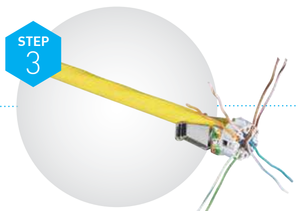
Separate and insert the pairs
