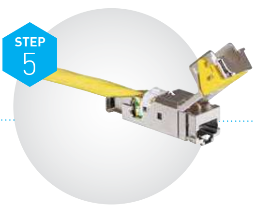
Install the wire housing without pushing
