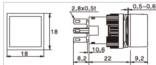
16mm Push Button Square- Illuminated
