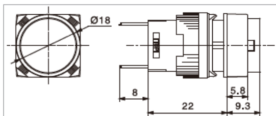
16mm Push Button Round - Illuminated
